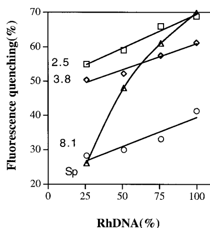
FIGURE 6 Fluorescence of 2.5 \mu\text{g} of Rh-DNA mixed with varying amounts of unlabelled DNA (percentage of Rh-DNA indicated on x axis) dissolved in \text{C}_{12}\text{E}_4 /TMP reverse micelles with W_o = 2.5 (square), 3.8 (diamond), and 8.1 (circle). The DNA in 25 mM HEPES pH 7.8, 0.5 mM was injected into 0.7 mL \text{C}_{12}\text{E}_4 /TMP. For control purposes, the same Rh-DNA mixtures were condensed with 2 mM spermine in HE buffer (triangle).
