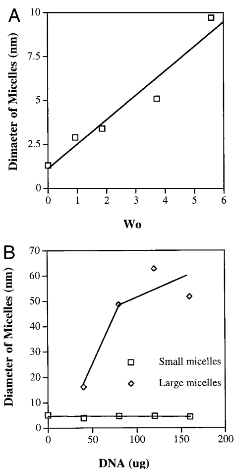
FIGURE 2 Size of w/o micelles using dynamic light scattering (particle size). (A) The dependence of the diameter of w/o micelles on water content without DNA. (B) At W_o = 3.54 , the effect of DNA concentration on the diameters of small micelles (presumably empty) and large micelles (presumably containing DNA).
